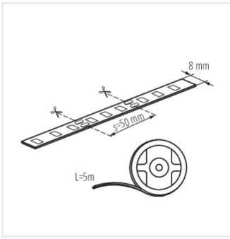
LEDS-B4,8W/M12IP00-NW
